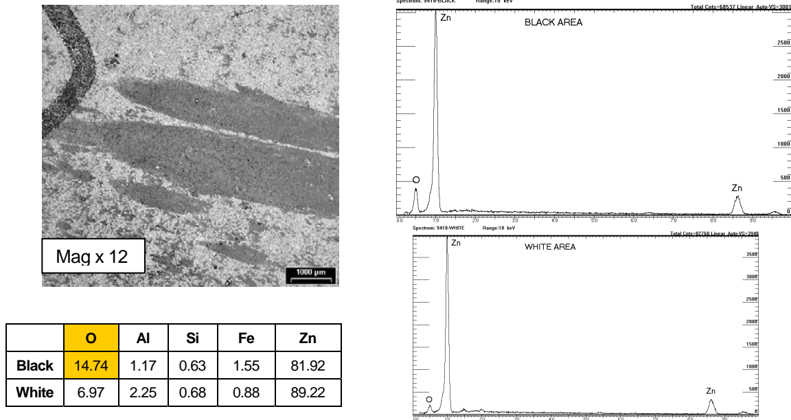
Figure 6 Analysis indicating black area has at least twice the oxygen content of the normal white zinc
